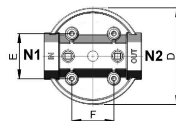
FFU N37 / FFU N47 Housing for DOE-filter cartridges (double open end)
