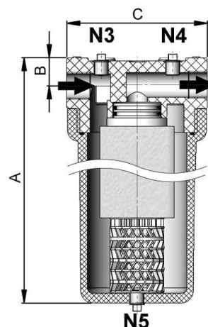
FFU N39 / FFU N48 Housing for adaptor filter cartridges with 222-O-ring (FFU N 39 for F2 / F3)
