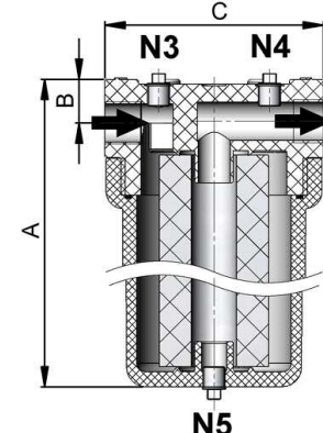
FFU N37 / FFU N47 Housing for DOE-filter cartridges (double open end)
