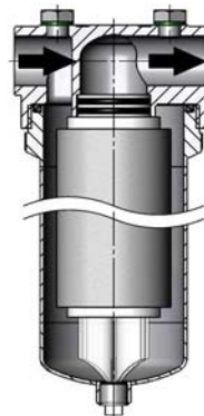
Installation situation with SOE-filter cartridge (Code 8) without adaptor
