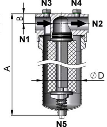
Installation situation with DOE-filter cartridge incl. support adaptor
